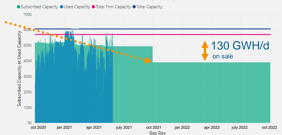
PIR Dunkirk : Subscribed and Used Capacity (MWh/d 0°C) by Gas Day
